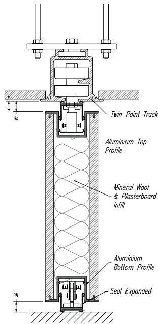
Twin Track Cross Section
