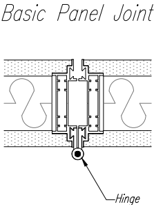
Typical M80 System - Cross Section
