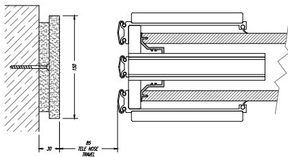
100 Slimline Telescopic Closer Detail
