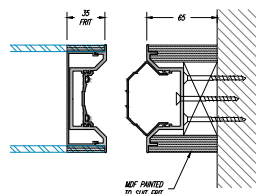
100 Slimline Scenic Basic Jamb Detail
