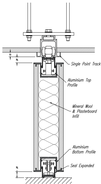
Single Point Track Cross Section
