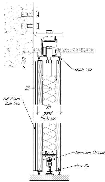
Single Point Cross Section
