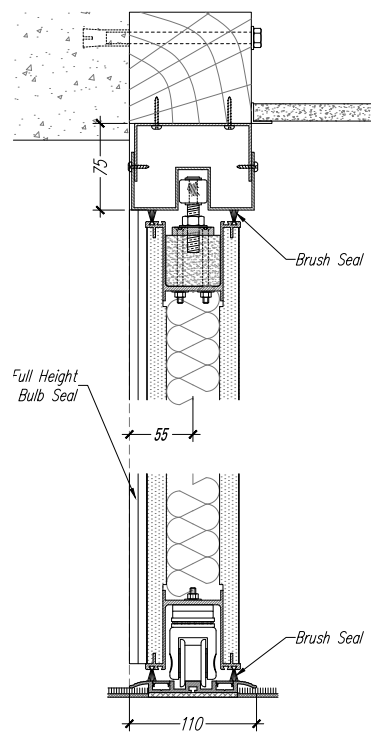
Bottom Rolling Cross Section
