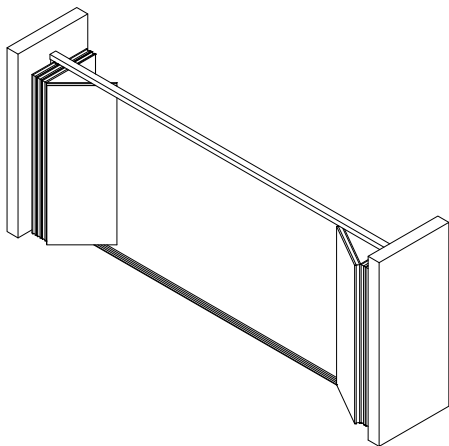
BP - 01 Bi-Parting Centre Fold
