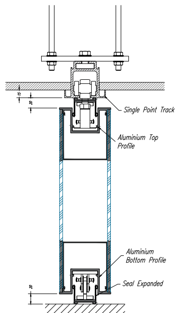
Single Track Cross Section
