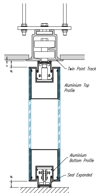
Twin Track Cross Section
