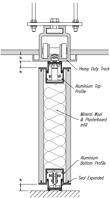
Heavy Duty Track Cross Section
