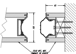
100 Slimline Basic Jamb Detail
