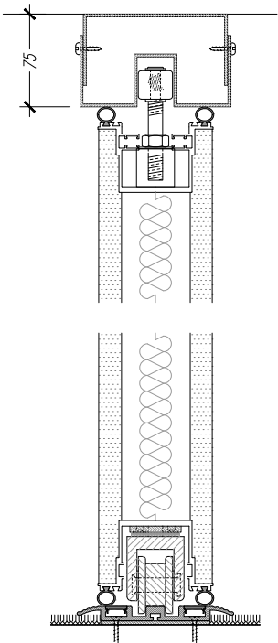
Bottom Rolling with Top Guide Cross Section
