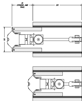
100 Slimline Scenic Expanding Jamb Detail
